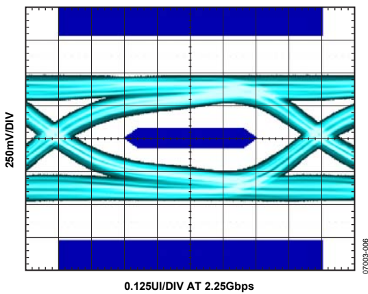
Figure 6. Rx Eye Diagram at TP2 (Cable = 6 m, 24 AWG)
